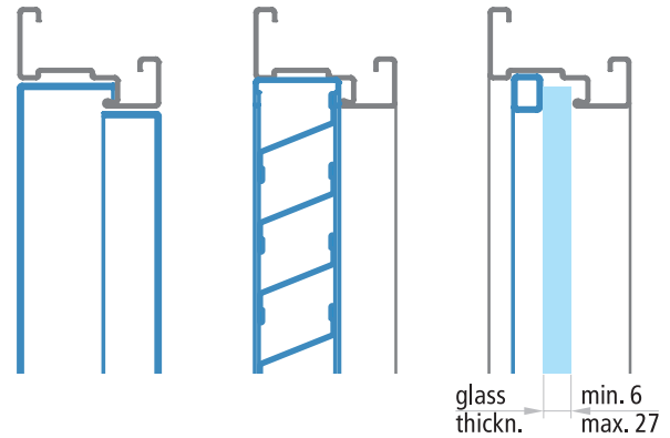
with glazing bead (glass not supplied)
