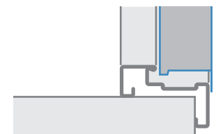
Leaf with lower rebate
