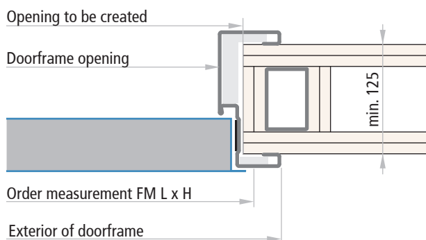
Door cross section and plasterboard version: REI 120 E 1,60 - E 1,120
