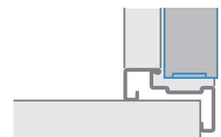
Leaf without lower rebate
