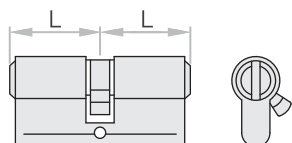
Nickel-plated cylinder equipped with 3 keys
