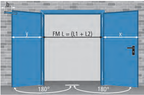
Two-leaved door
