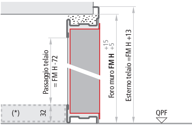
Doors with internal lower threshold Vertical cross section
