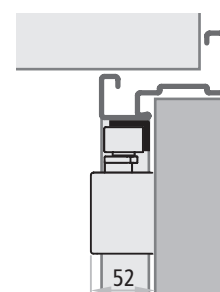
CP2-G PROGET (from push side)
