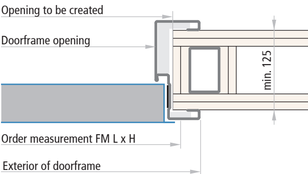
Door cross section and plasterboard version: REI 120 EI 2 60 - EI 2 120
