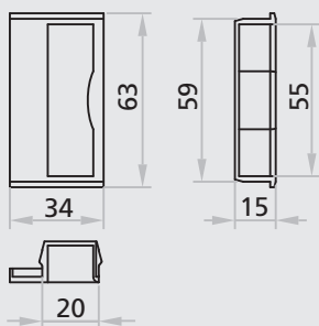
Strike box lock insert for one-leaved doors of PROGET and other multipurpose doors
