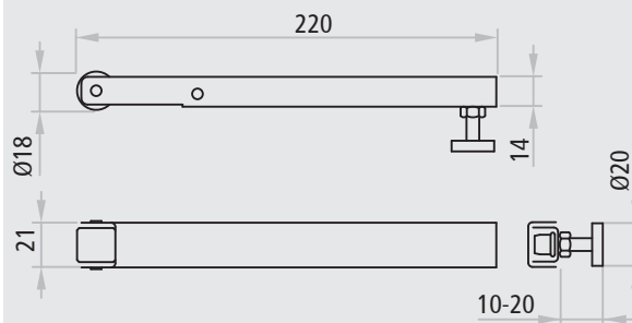
Carrier arm for inactive leaf
