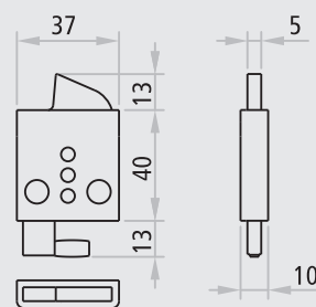
Upper re-latch device for inactive leaf of UNIVER and REVER
