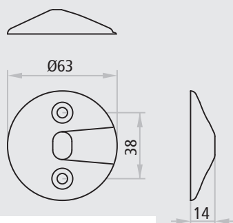
Lower floor catch for inactive leaf of UNIVER
