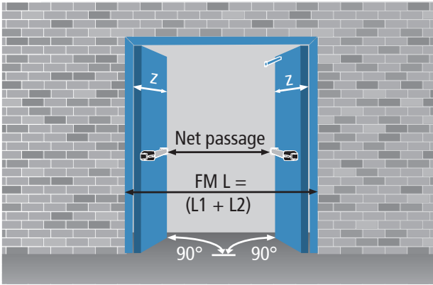
Two-leaved doors with panic bars
