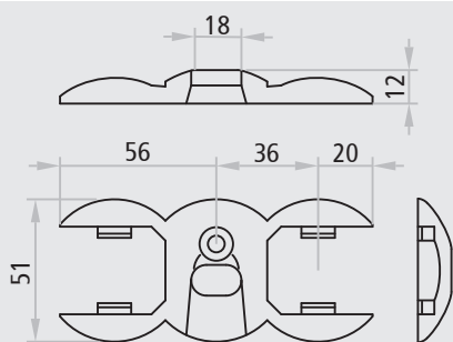
Lower floor catch for inactive leaf of REVER
