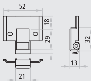
Upper strike box for inactive leaf of PROGET and other multipurpose doors
