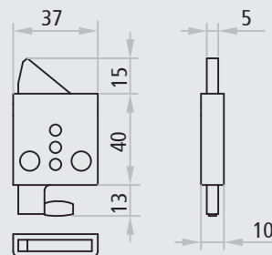
Upper re-latch device for inactive leaf of PROGET and other multipurpose doors
