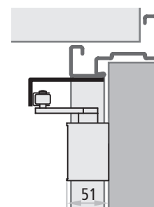
CP1-G PROGET (from push side)
