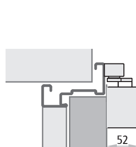
CP2 PROGET (from pull side)
