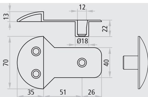
Lower floor catch for inactive leaf of PROGET and other multipurpose doors
